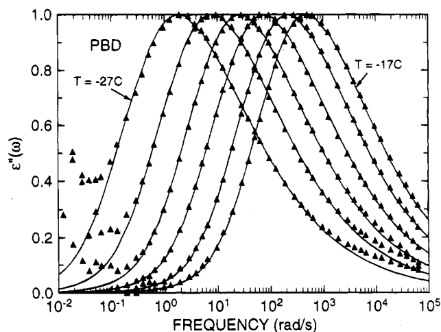
Figure 3. Isothermal segmental relaxation peak in the dielectric loss of PBD displayed at 2^\circ\text{C} increments from -27 to -17^\circ\text{C} . The peak broadens with decreasing temperature (e.g., best fit \beta = 0.43 at the highest and 0.39 at the lowest temperature).
